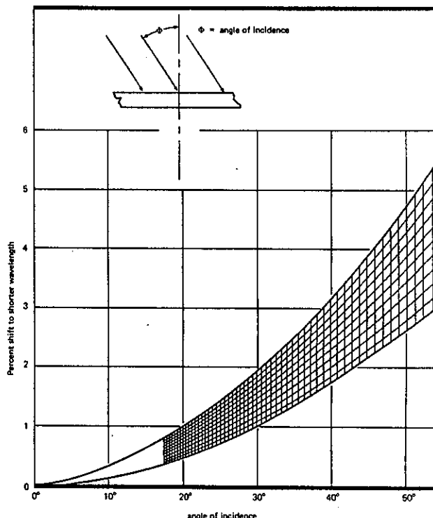
Wavelength Shift of Interference Filters as a Function of Angle of Incidence Collimated Radiation
