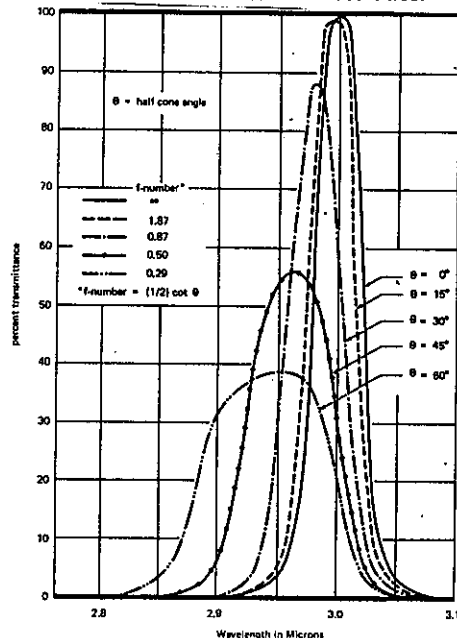
Variation of Spectral Characteristics with F - Number on 1.4% Filter
