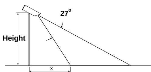
Figure 1.3 - Vertical field-of-view (grounded)
